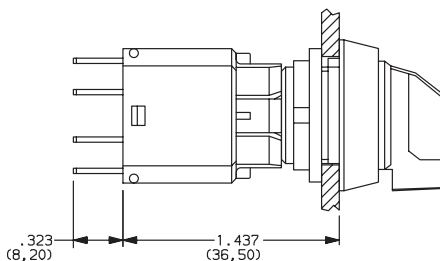
Contact Block with Momentary and Latching Selector Switch
